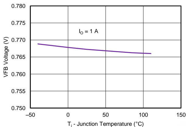
Figure 12. VFB VOLTAGE vs JUNCTION TEMPERATURE ( I_O = 1\text{ A} )
