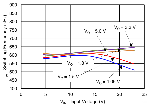
Figure 10. SWITCHING FREQUENCY vs INPUT VOLTAGE ( I_O = 1\text{ A} )
