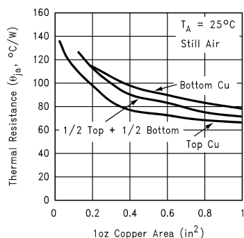
FIGURE 7. \theta_{JA} vs. 1oz Copper Area for SOT-223
