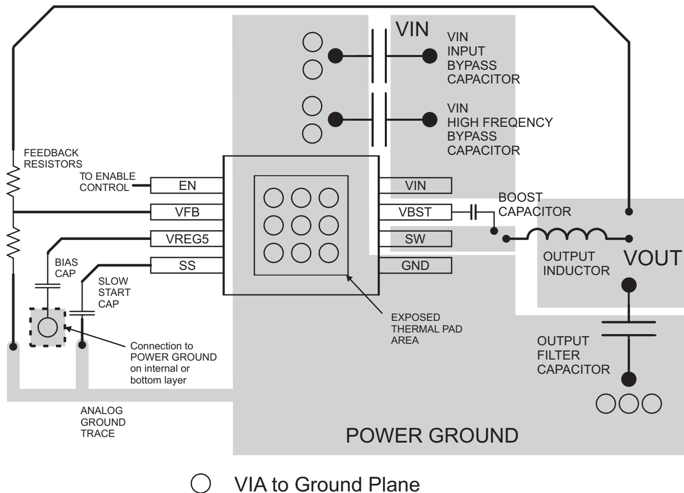
Figure 17. PCB Layout
