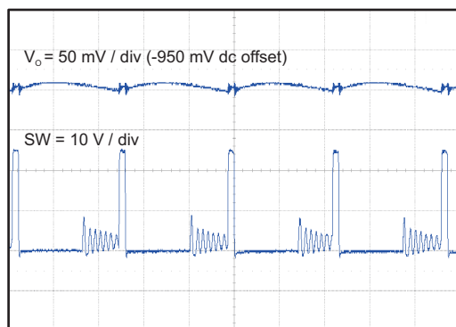
Figure 13. DCM VOLTAGE RIPPLE AT OUTPUT ( I_O = 30 \text{ mA} )
