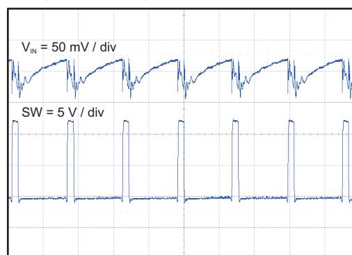
Figure 14. VOLTAGE RIPPLE AT INPUT ( I_O = 3 \text{ A} )
