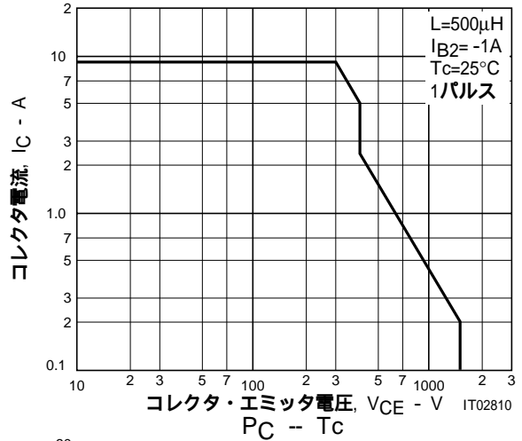
Reverse Bias A S O
